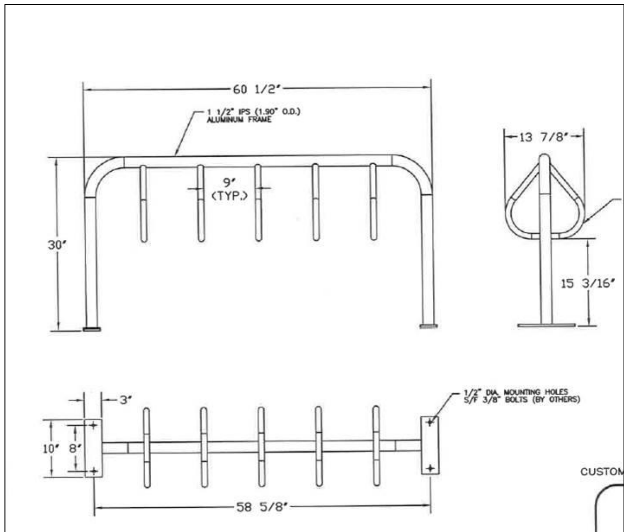
Bike rack dimensions
